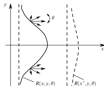
Figure 1. Intensity function in a two-dimensional problem.
