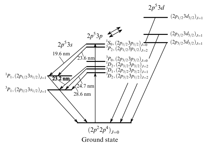
Figure 1. Energy level diagram of the Ne-like Ge XXII ion illustrating the main processes of excitation and radiative decay resulting in the inversion on the 3p - 3s transition. The wavelengths of laser transitions are indicated.
