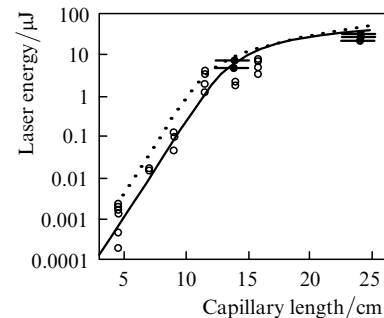
Figure 8. Dependence of the lasing energy on the capillary length: comparison of calculations (horizontal bars) with experiment (circles).
