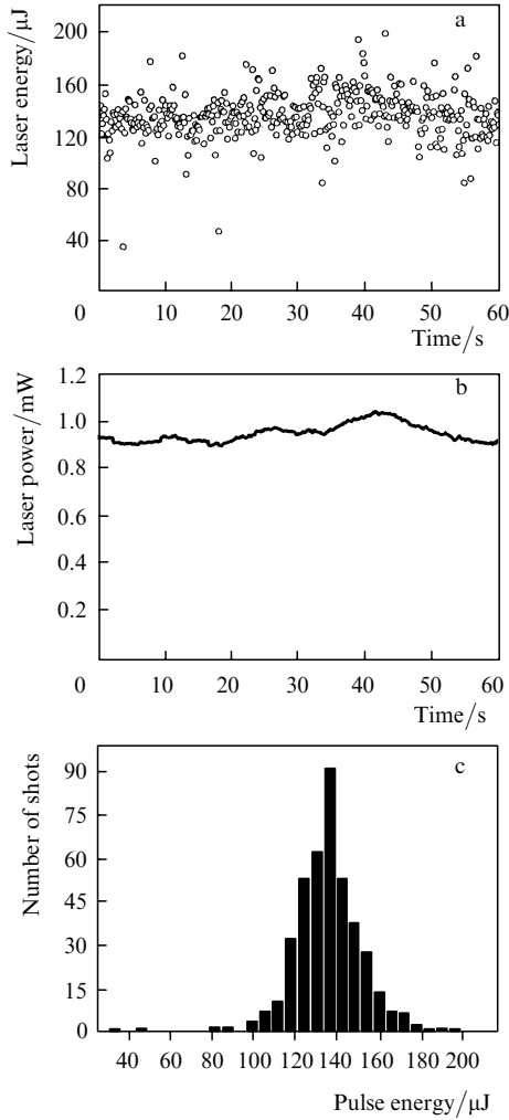
Figure 9. Energy characteristics of the 469-Å laser with a pulse repetition rate of 4 Hz: time dependence of the pulse energy (a), the pulse power averaged over 60 shots (b), and the energy distribution of pulses (c).
