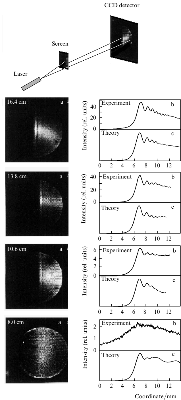
Figure 11. Scheme and the results of measurements of the spatial coherence of the capillary discharge laser. At the left: (a) diffraction patterns obtained for different capillary lengths; at the right: results of the pattern processing (b) and simulations (c).
