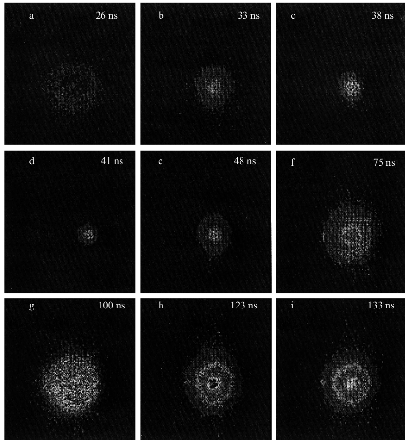
Figure 5. Sequence of images of a capillary plasma (view from the end); a capillary of diameter 4 mm and length 12 cm is filled with Ar at a pressure of 700 mTorr, the discharge current is 39 kA, the half-period duration is 62 ns. The images corresponding to a maximum compression (d, e) were obtained at a reduced sensitivity of a detector.
