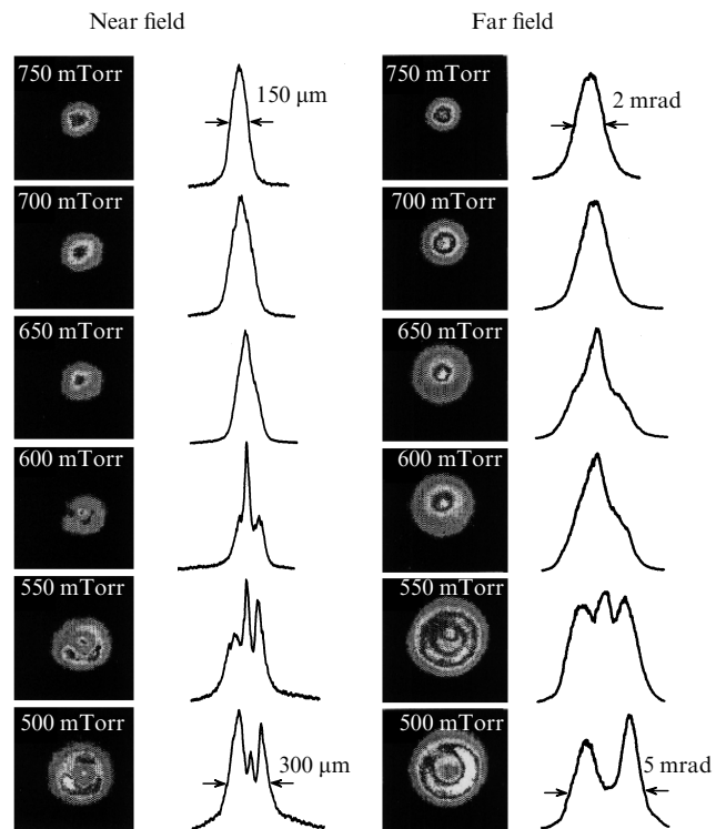
Figure 10. Near- and far-field radiation intensity distributions for the X-ray laser at argon pressures varied from 500 to 750 mTorr.
