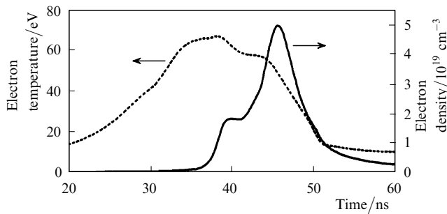
Figure 6. Calculated behaviour of the electron density and temperature at the capillary-discharge axis.
