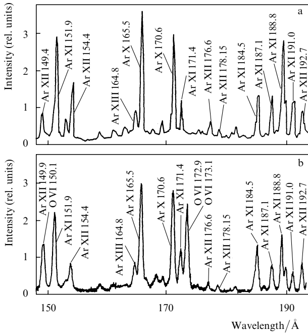
Figure 4. X-ray spectra of Ar obtained on the high-power Gamble II facility at a current of 1 MA and a few terawatt power (a) and in a capillary discharge of diameter 2.5 mm at a current of 43 kA and a current pulse duration (FWHM) of 30 ns (b).
