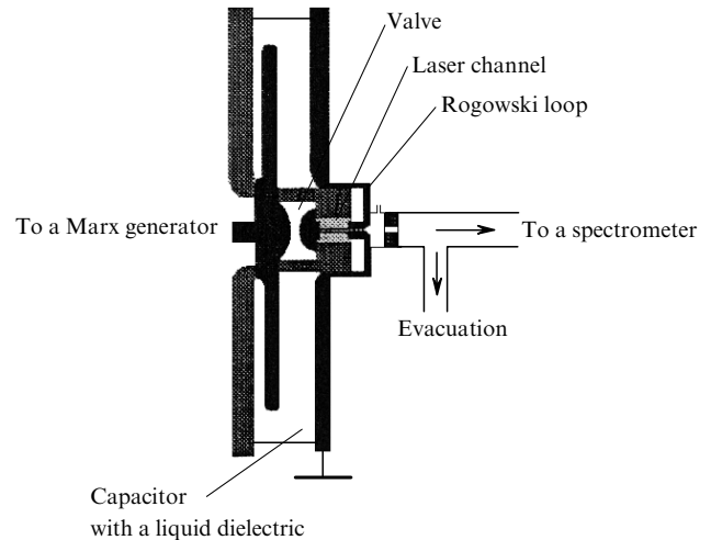
Figure 2. Scheme of a capillary discharge for producing lasing at 469 Å in the Ne-like Ar in the saturation regime [42, 43].
