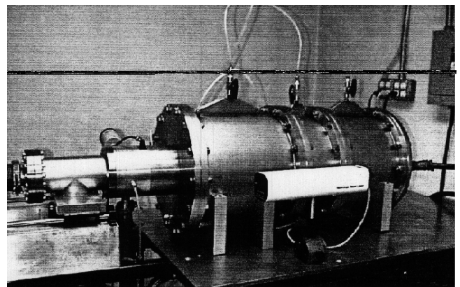
Figure 3. Capillary discharge X-ray laser with an average output power of \sim 1 \text{ mW} . For comparison, a 5-mW helium-neon laser is shown in front of the X-ray laser (photo courtesy of the Colorado State University).
