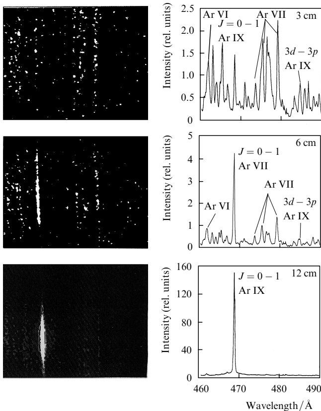
Figure 7. Spectra observed along the capillary-discharge axis. The increase in the 469-Å line intensity with increasing the capillary length from 3 to 12 cm clearly demonstrates laser action.
