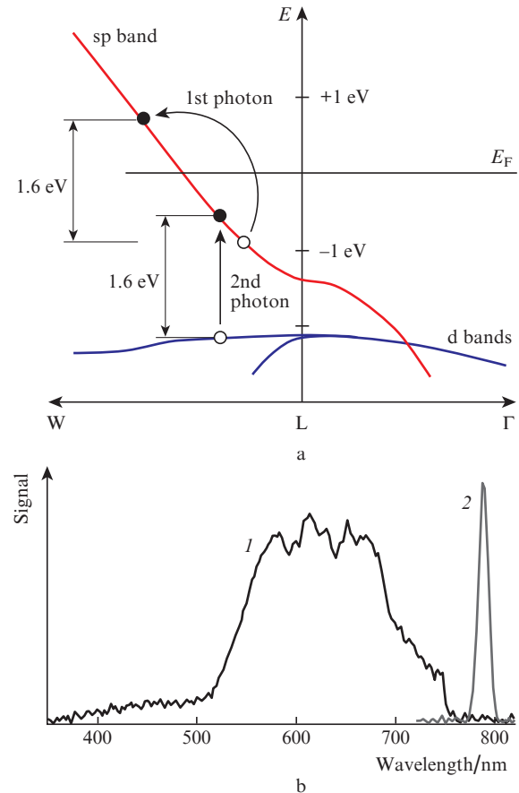
Figure 4. (Colour online) Two-photon luminescence in gold: (a) schematic of the gold band structure near the symmetry point L of the first Brillouin zone (multiphoton excitation transfers an electron from the d band to the sp band and (b) measured 2PPL spectrum (1) and laser excitation spectrum (2).
