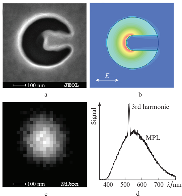
Figure 5. (Colour online) Multiphoton photoluminescence (MPL) from an SHR nanostructure fabricated in a 50-nm-thick aluminium film: (a) electron microscopy image of the nanostructure; (b) calculated field distribution in the nanostructure irradiated by a plane monochromatic wave with \lambda = 1560 nm; (c) optical image of the nanostructure illuminated by a laser with \lambda = 1560 nm, recorded in the spectral range of 400–800 nm; and (d) measured MPL spectrum of the nanostructure illuminated by a laser with \lambda = 1560 nm.
